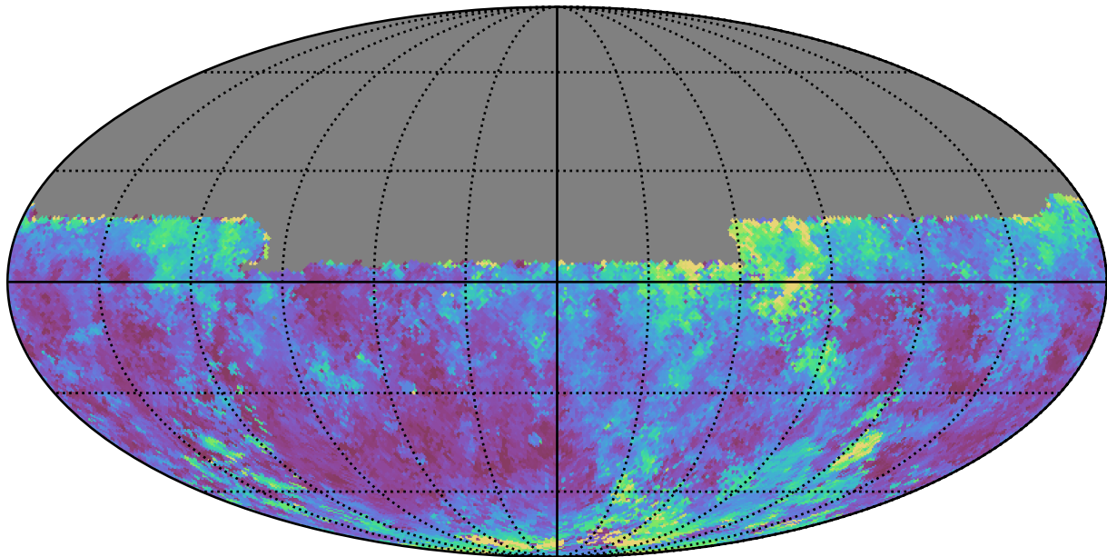
too_100_1v3.4_10yrs Yr 1 y band: Median seeingGeom
