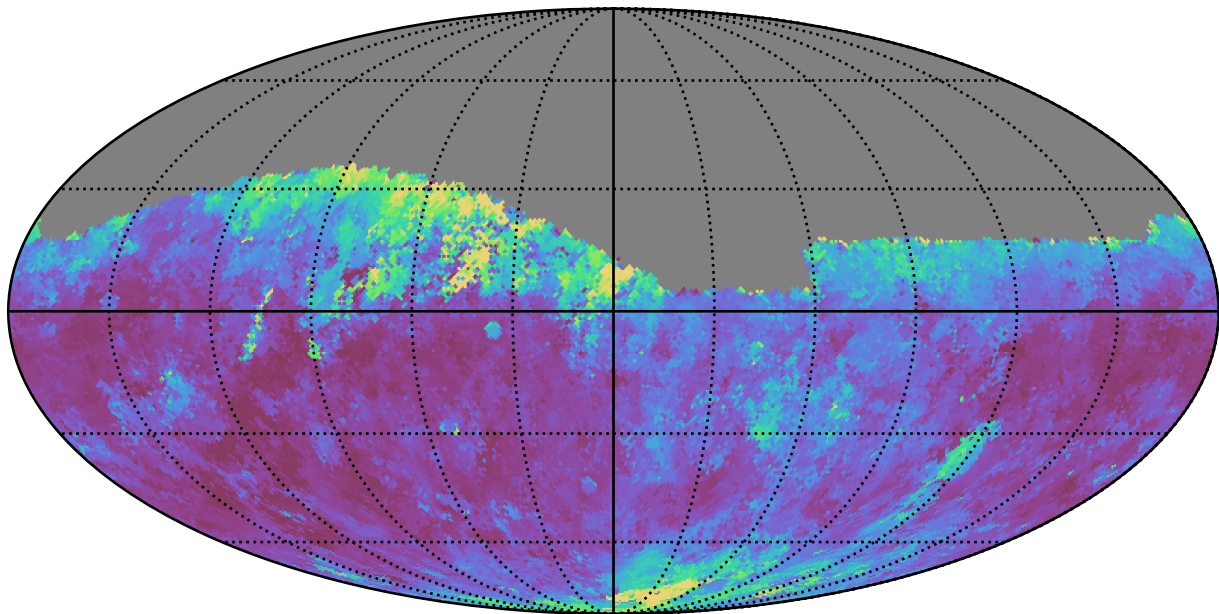
too_100_1v3.4_10yrs Yr 1 r band: Median seeingGeom
