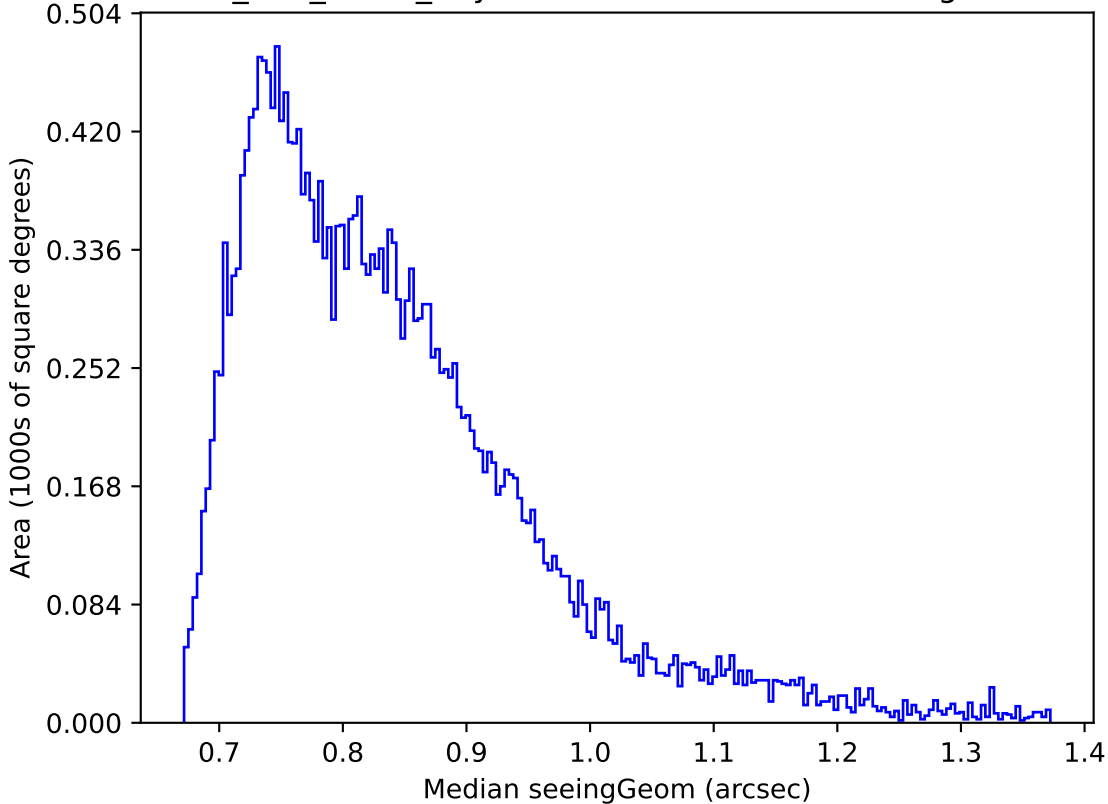
too_100_1v3.4_10yrs Yr 1 i band: Median seeingGeom
