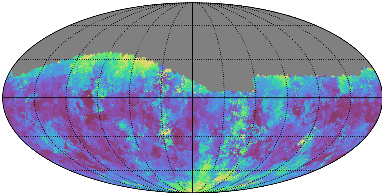
too_100_1v3.4_10yrs Yr 1 g band: Median seeingGeom
