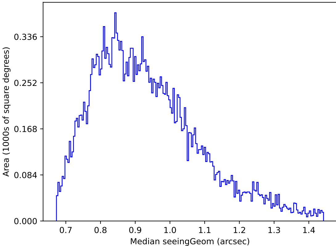
too_100_1v3.4_10yrs Yr 1 g band: Median seeingGeom
