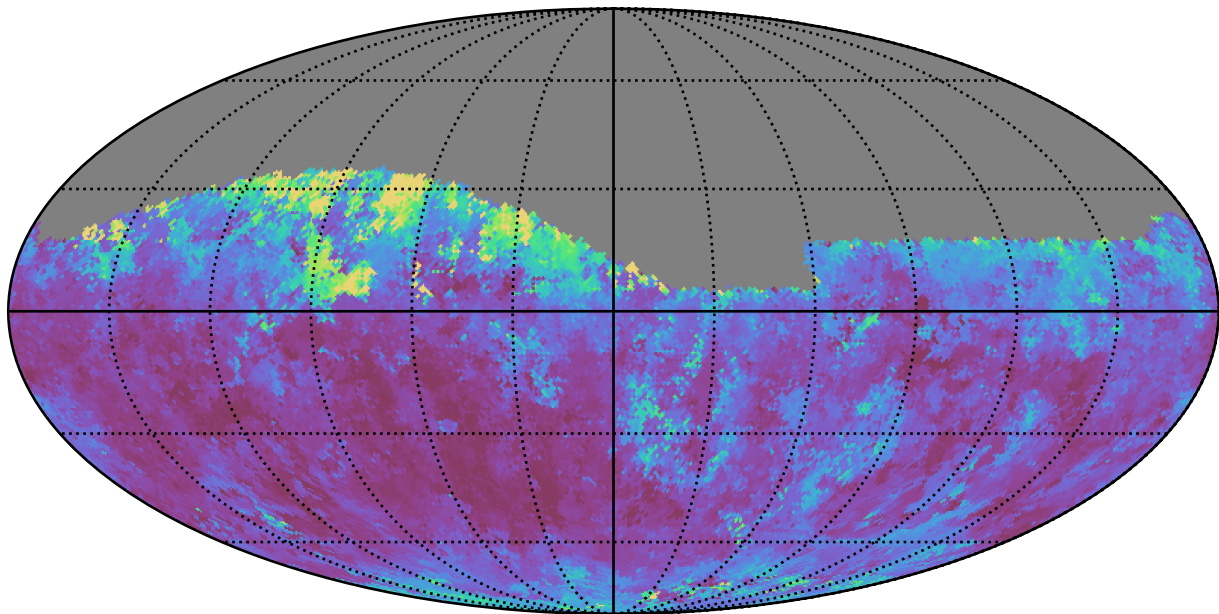
too_100_1v3.4_10yrs Yr 1 z band: Median seeingEff
