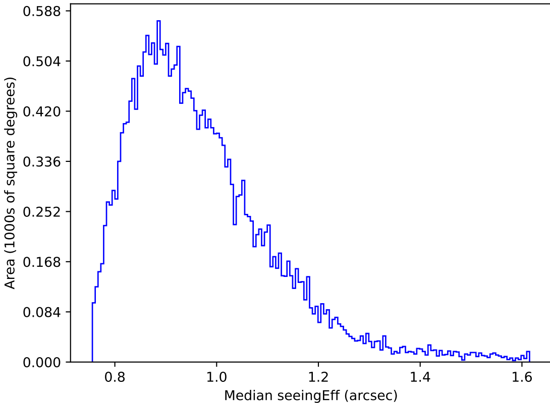
too_100_1v3.4_10yrs Yr 1 z band: Median seeingEff
