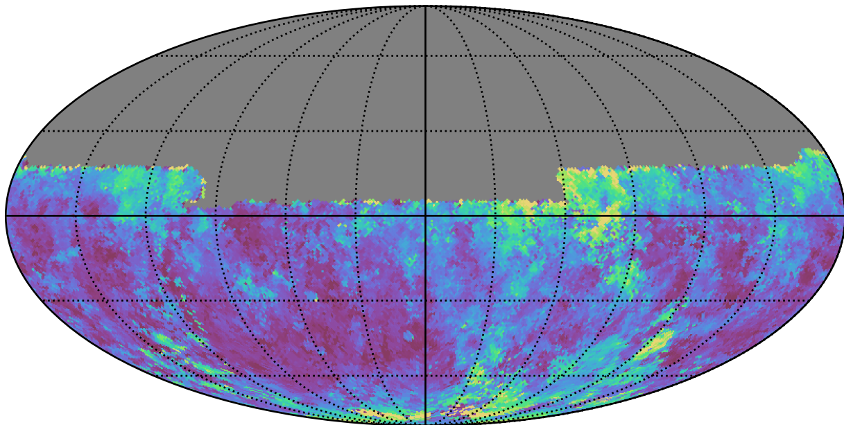
too_100_1v3.4_10yrs Yr 1 y band: Median seeingEff
