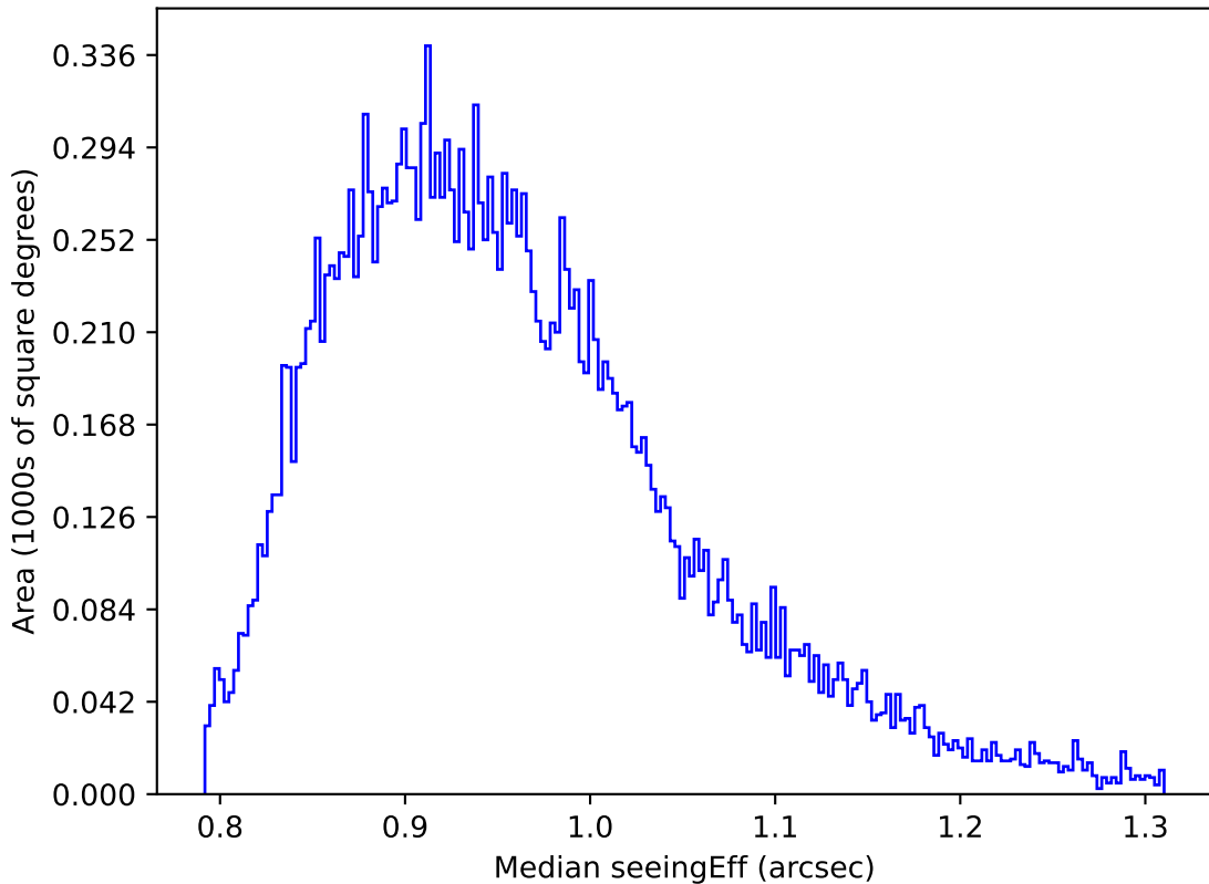
too_100_1v3.4_10yrs Yr 1 y band: Median seeingEff
