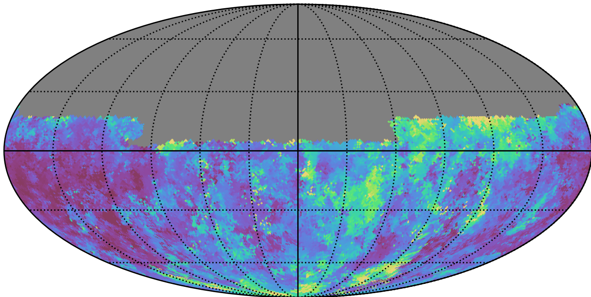
too_100_1v3.4_10yrs Yr 1 u band: Median seeingEff
