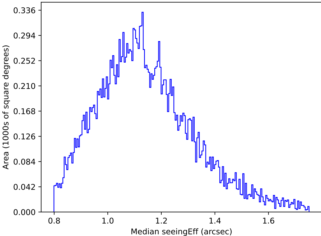
too_100_1v3.4_10yrs Yr 1 u band: Median seeingEff
