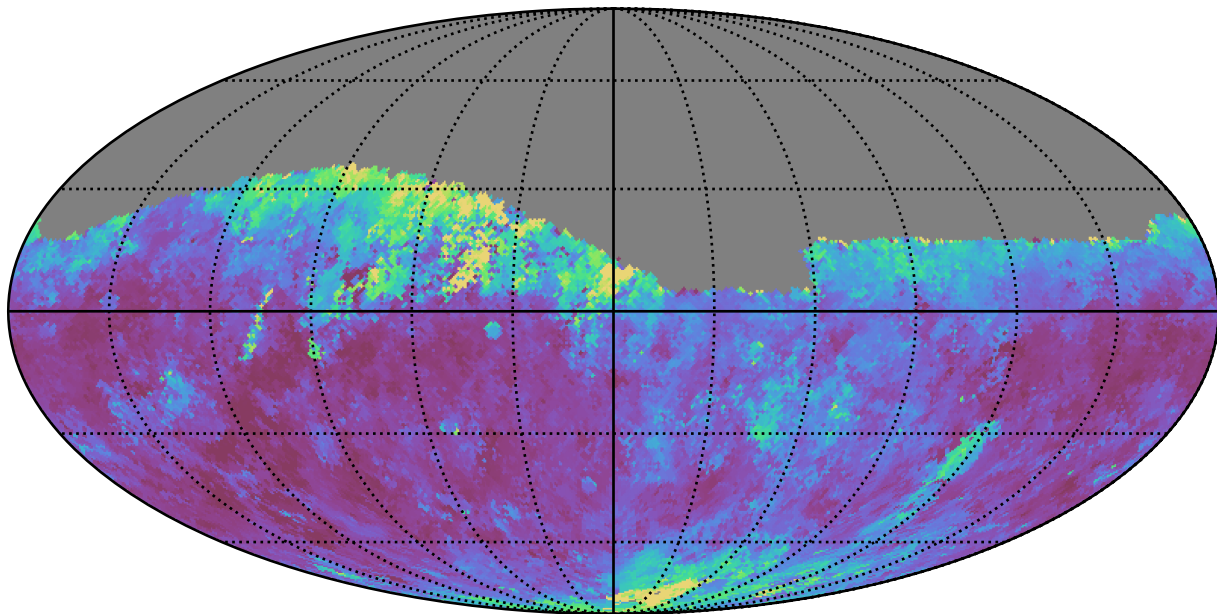
too_100_1v3.4_10yrs Yr 1 r band: Median seeingEff
