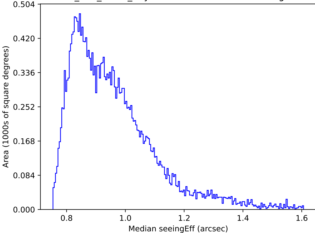
too_100_1v3.4_10yrs Yr 1 i band: Median seeingEff
