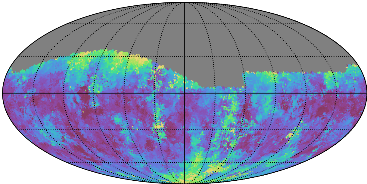
too_100_1v3.4_10yrs Yr 1 g band: Median seeingEff
