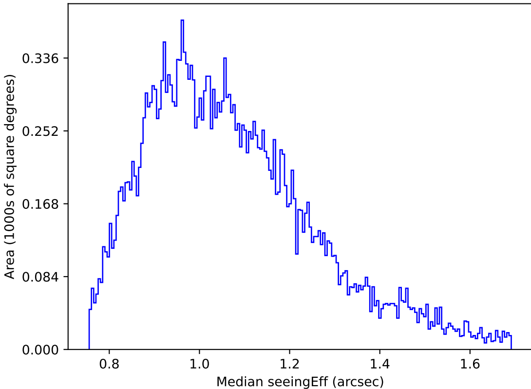
too_100_1v3.4_10yrs Yr 1 g band: Median seeingEff
