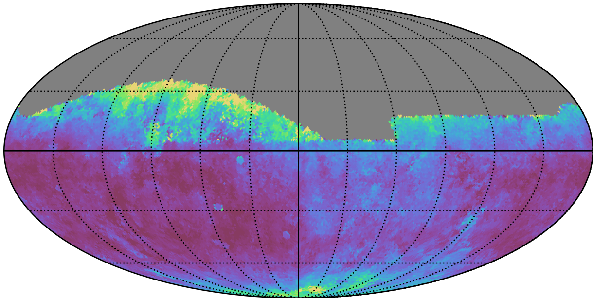
too_100_1v3.4_10yrs Yr 1 all bands: Median seeingEff
