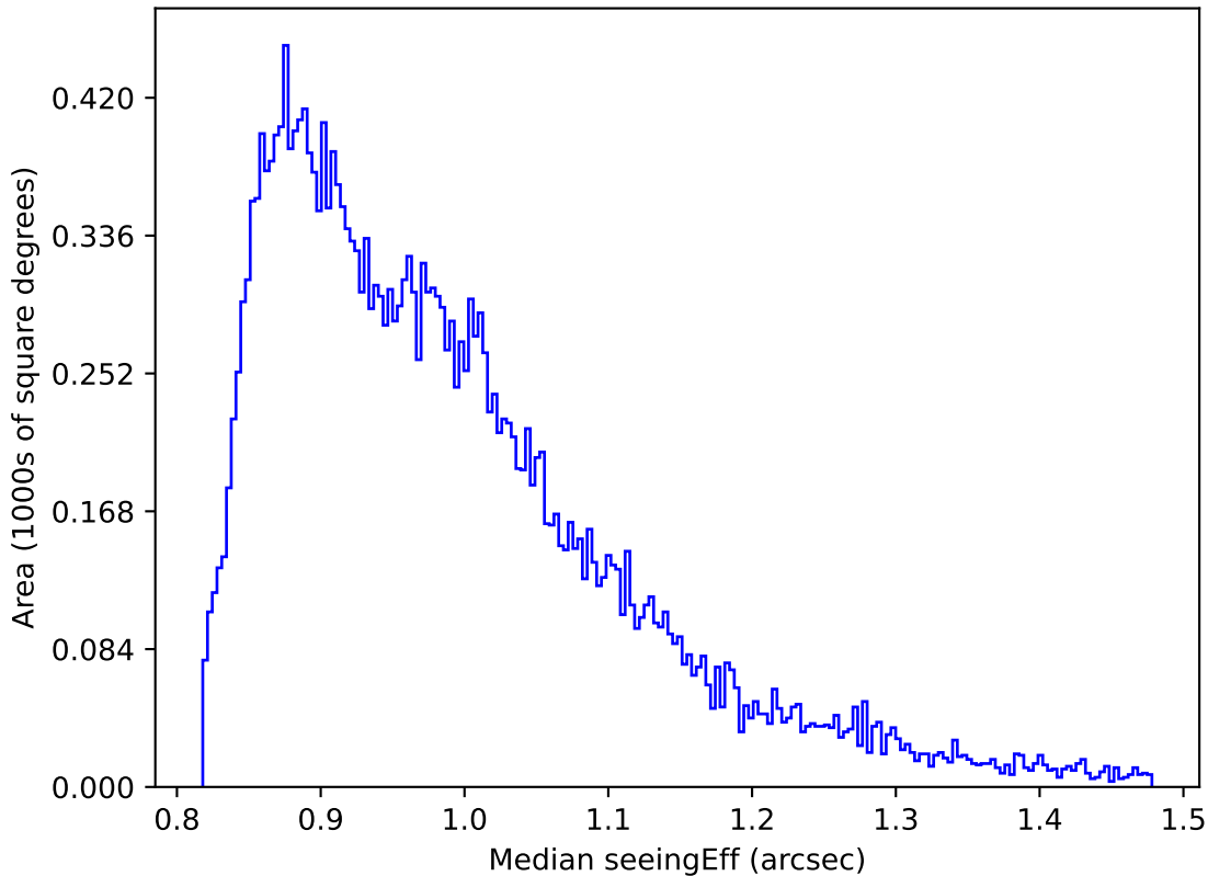
too_100_1v3.4_10yrs Yr 1 all bands: Median seeingEff
