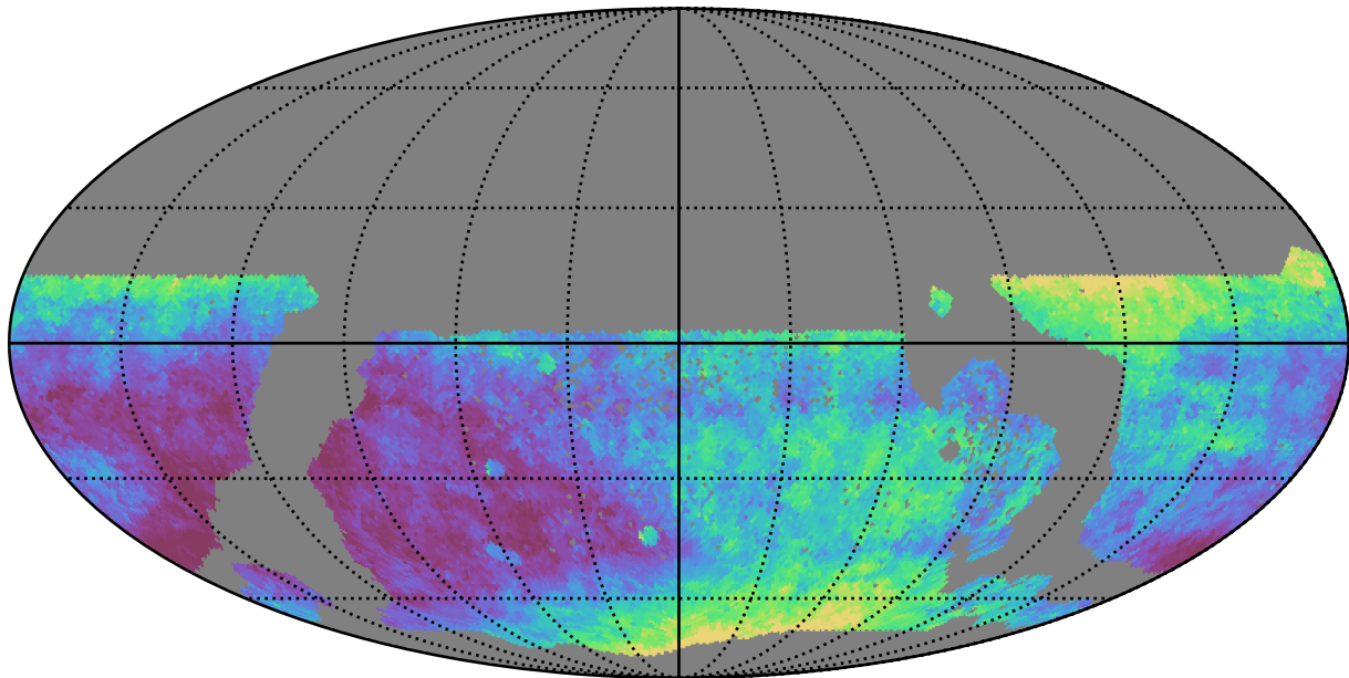
too_100_1v3.4_10yrs WFD z band: Median seeingEff
