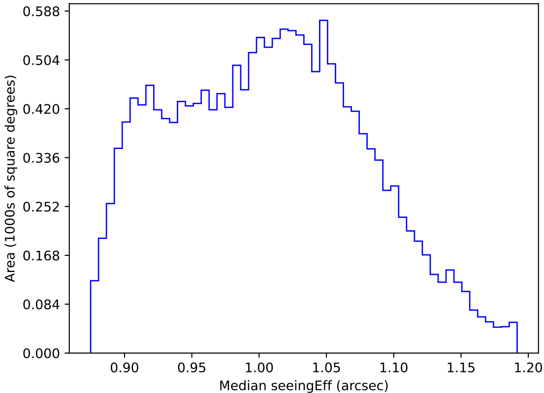
too_100_1v3.4_10yrs WFD z band: Median seeingEff
