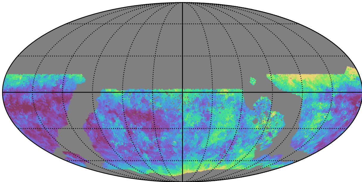
too_100_1v3.4_10yrs WFD u band: Median seeingEff
