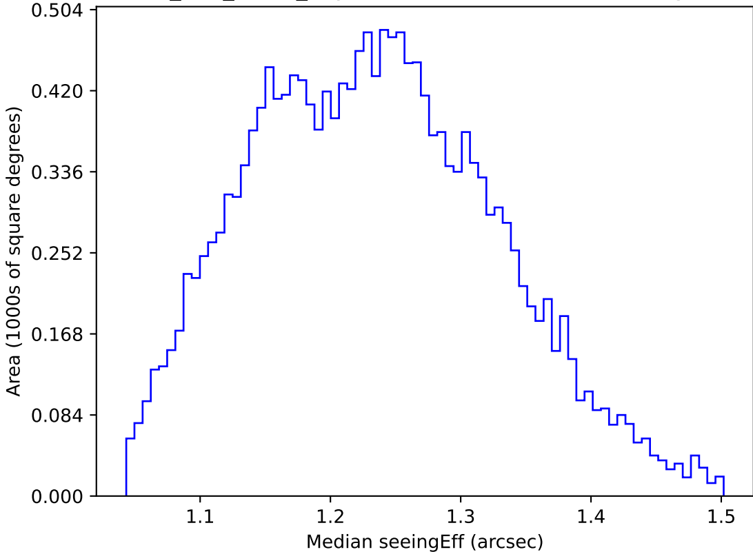
too_100_1v3.4_10yrs WFD u band: Median seeingEff
