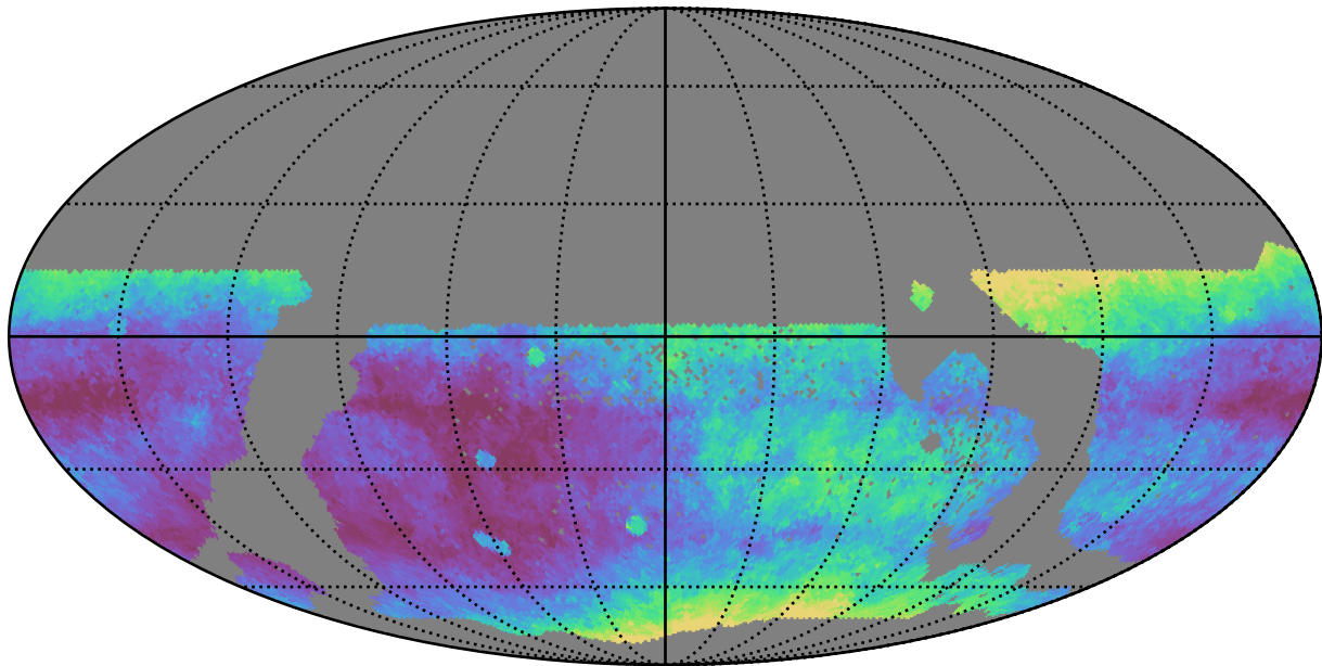
too_100_1v3.4_10yrs WFD r band: Median seeingEff
