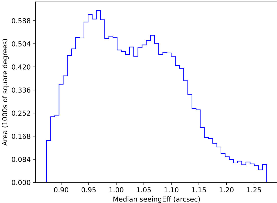
too_100_1v3.4_10yrs WFD r band: Median seeingEff
