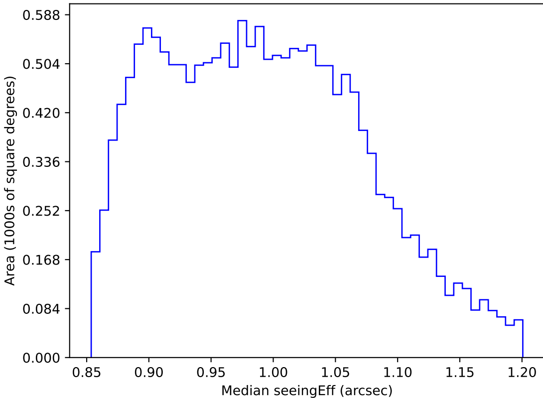
too_100_1v3.4_10yrs WFD i band: Median seeingEff
