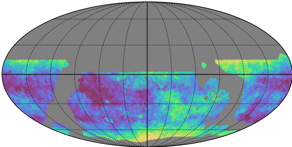
too_100_1v3.4_10yrs WFD g band: Median seeingEff
