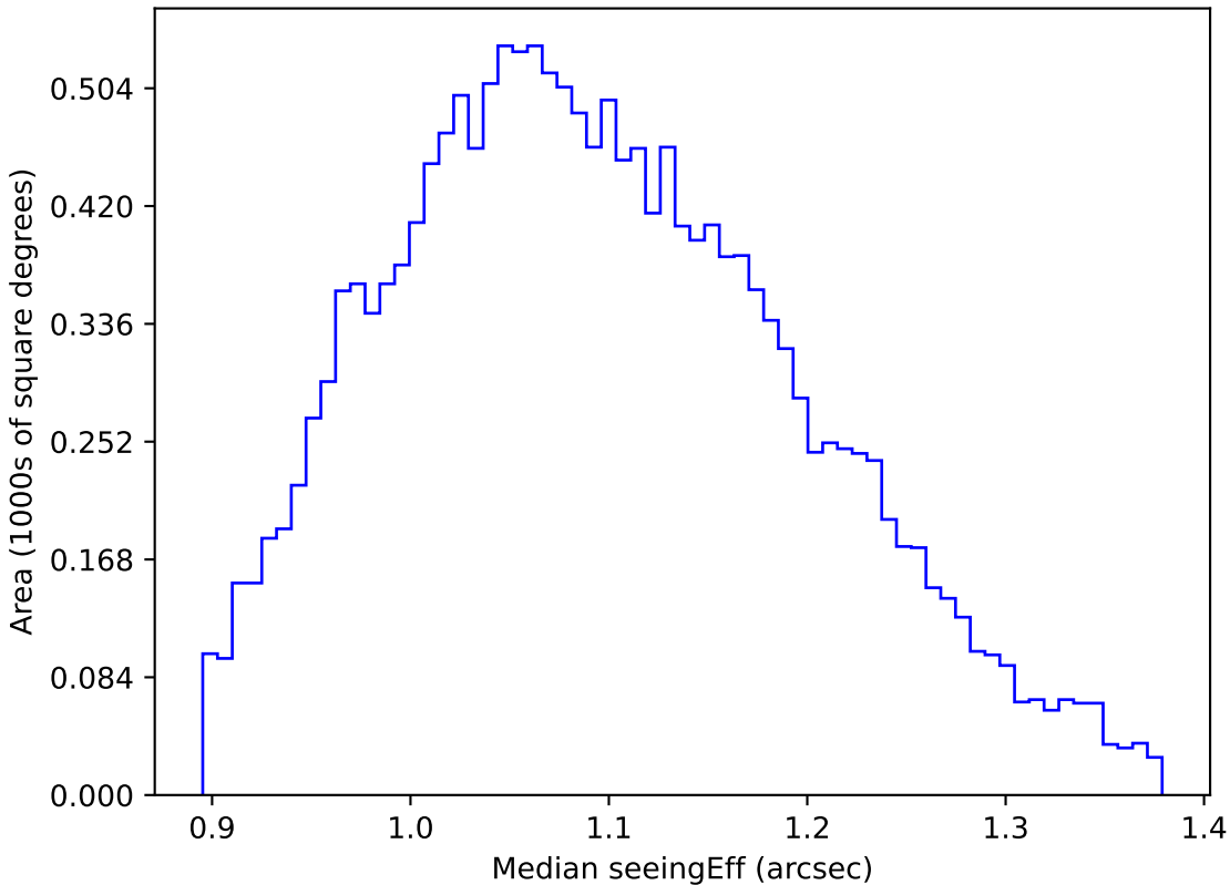
too_100_1v3.4_10yrs WFD g band: Median seeingEff
