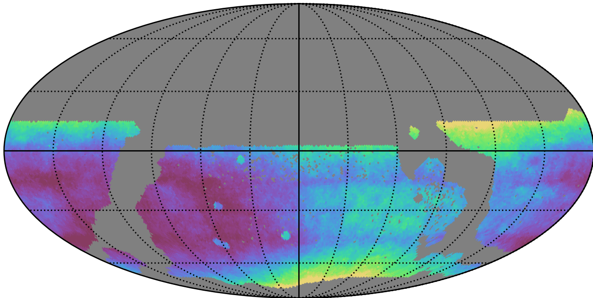
too_100_1v3.4_10yrs WFD all bands: Median seeingEff
