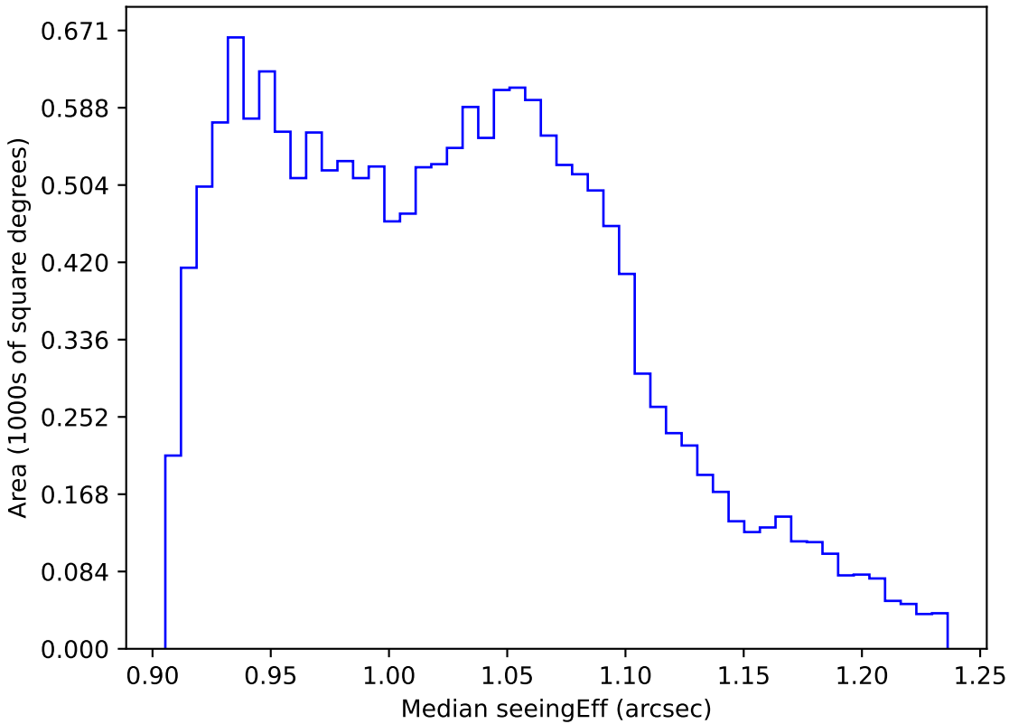
too_100_1v3.4_10yrs WFD all bands: Median seeingEff
