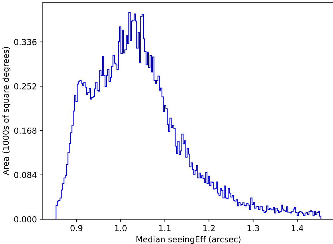
too_100_1v3.4_10yrs All sky z band: Median seeingEff
