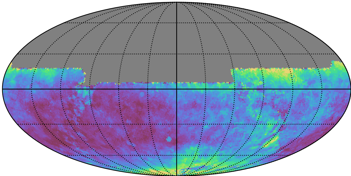
too_100_1v3.4_10yrs All sky y band: Median seeingEff
