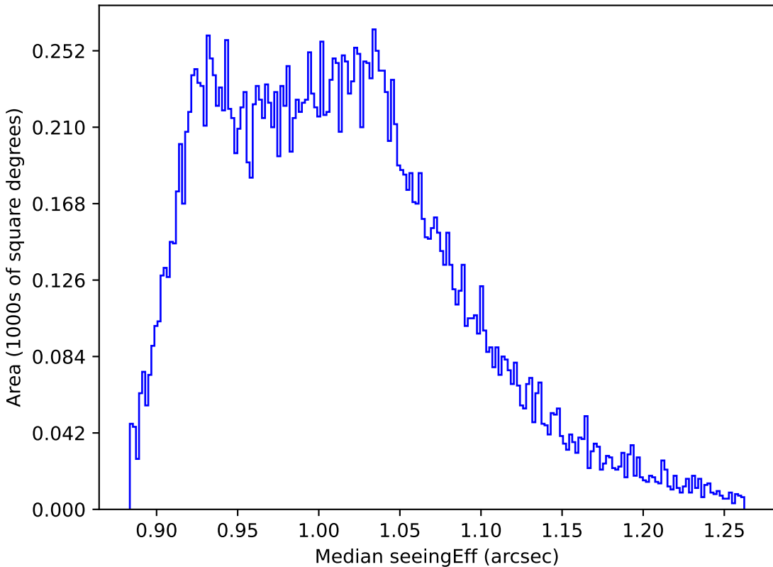
too_100_1v3.4_10yrs All sky y band: Median seeingEff
