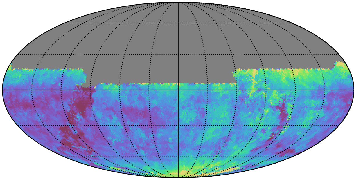
too_100_1v3.4_10yrs All sky u band: Median seeingEff
