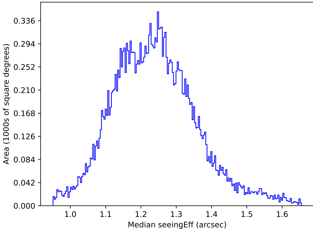
too_100_1v3.4_10yrs All sky u band: Median seeingEff
