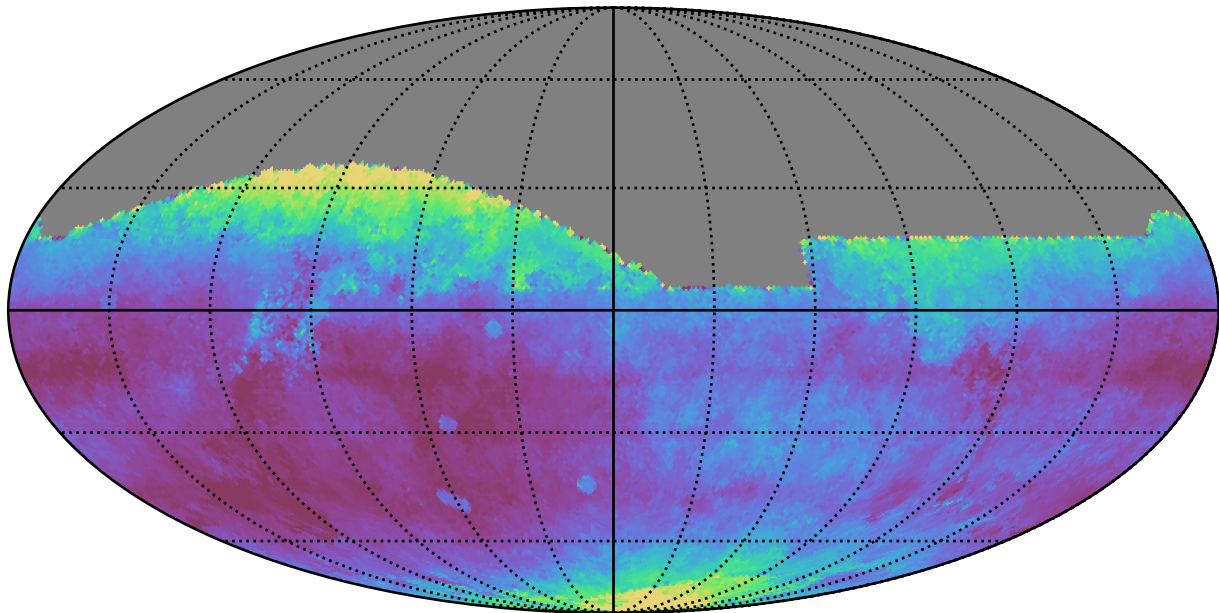
too_100_1v3.4_10yrs All sky r band: Median seeingEff
