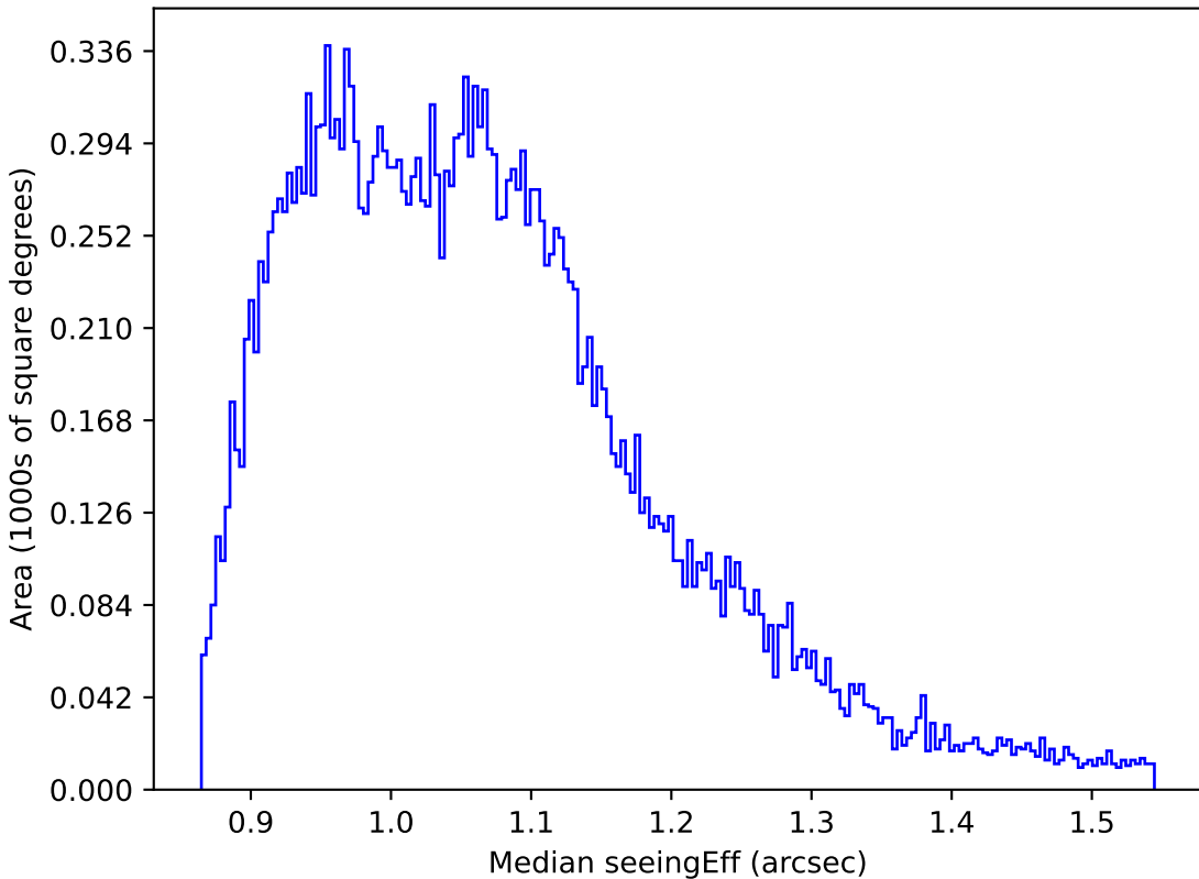
too_100_1v3.4_10yrs All sky r band: Median seeingEff
