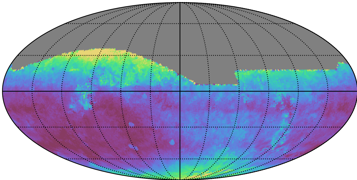
too_100_1v3.4_10yrs All sky i band: Median seeingEff
