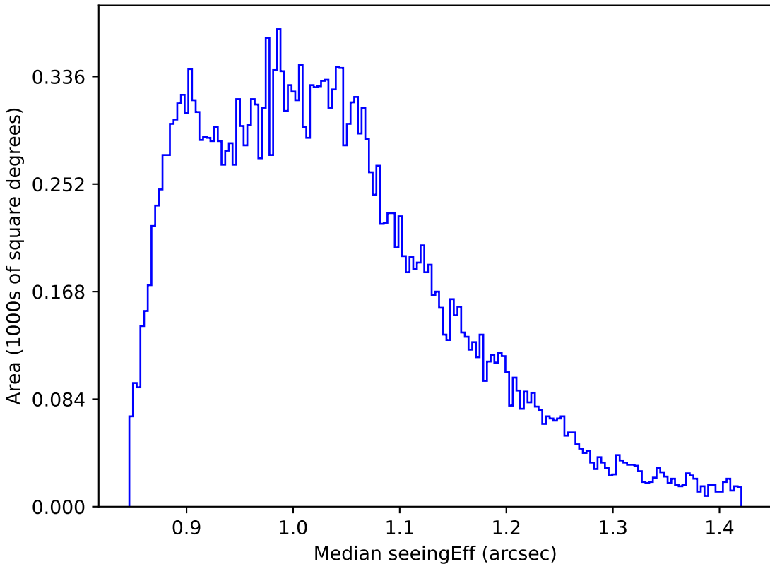
too_100_1v3.4_10yrs All sky i band: Median seeingEff
