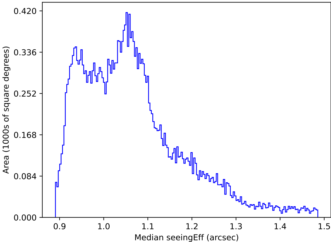
too_100_1v3.4_10yrs All sky all bands: Median seeingEff
