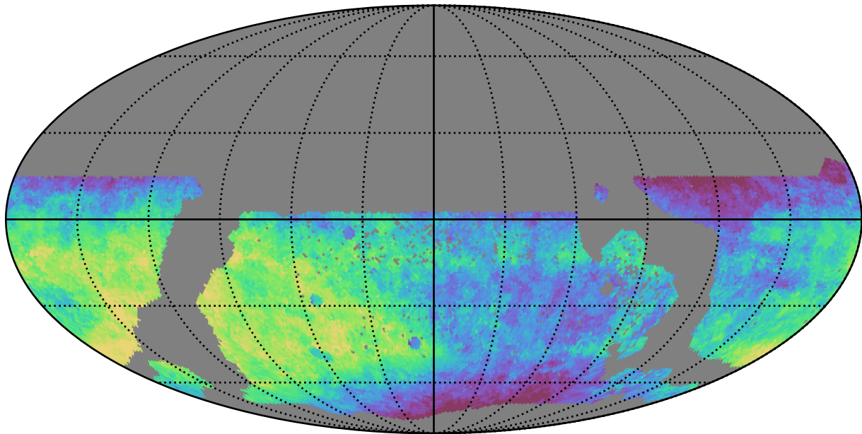
too_100_1v3.4_10yrs WFD z band: Median saturation_mag
