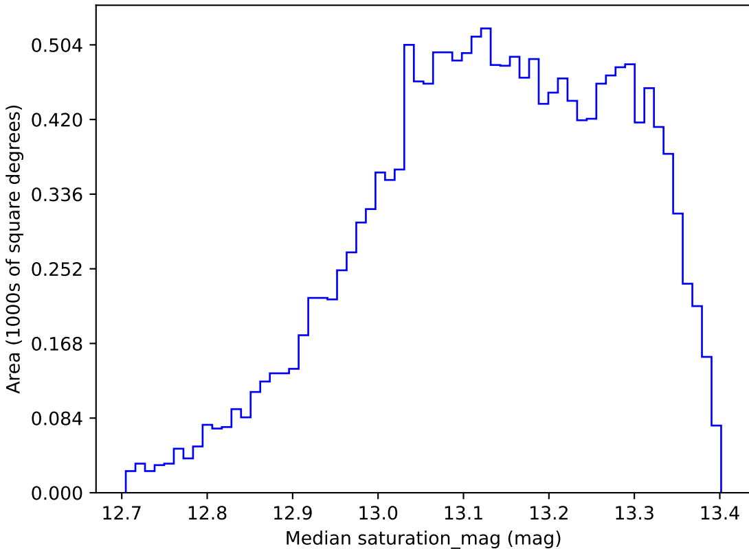
too_100_1v3.4_10yrs WFD y band: Median saturation_mag
