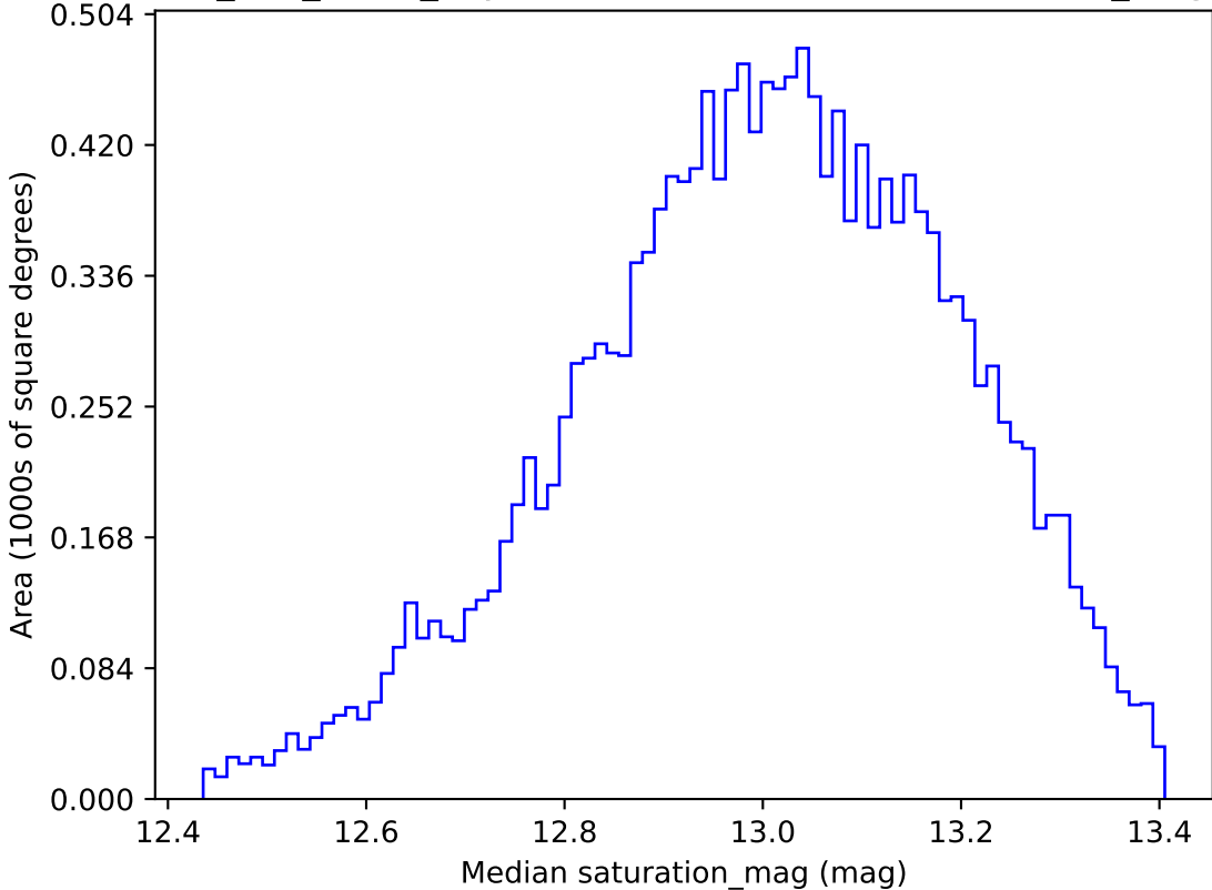
too_100_1v3.4_10yrs WFD u band: Median saturation_mag
