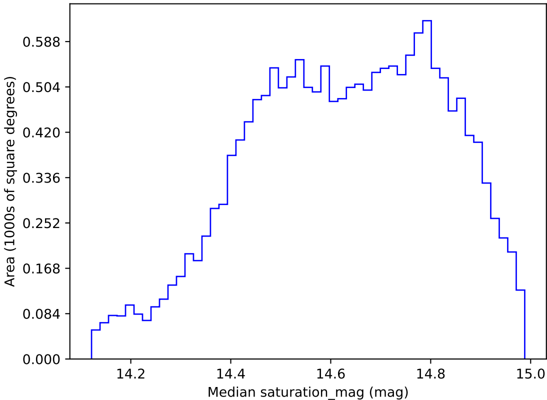
too_100_1v3.4_10yrs WFD r band: Median saturation_mag
