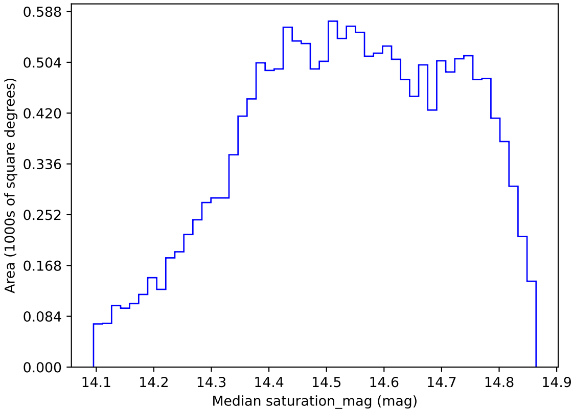
too_100_1v3.4_10yrs WFD i band: Median saturation_mag
