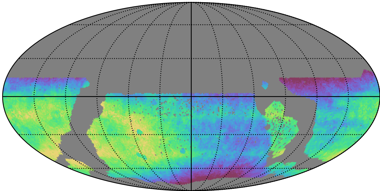
too_100_1v3.4_10yrs WFD all bands: Median saturation_mag
