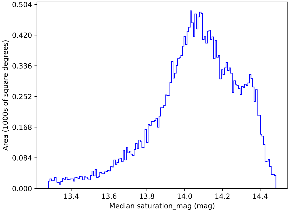
too_100_1v3.4_10yrs All sky z band: Median saturation_mag
