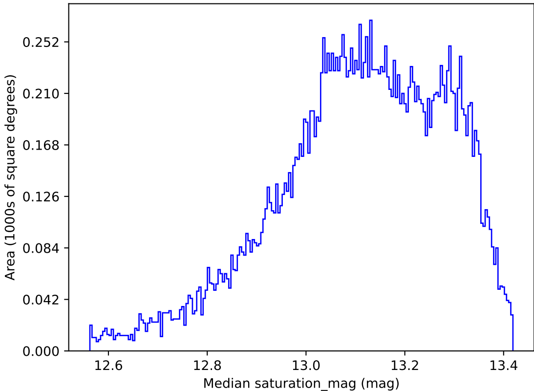
too_100_1v3.4_10yrs All sky y band: Median saturation_mag
