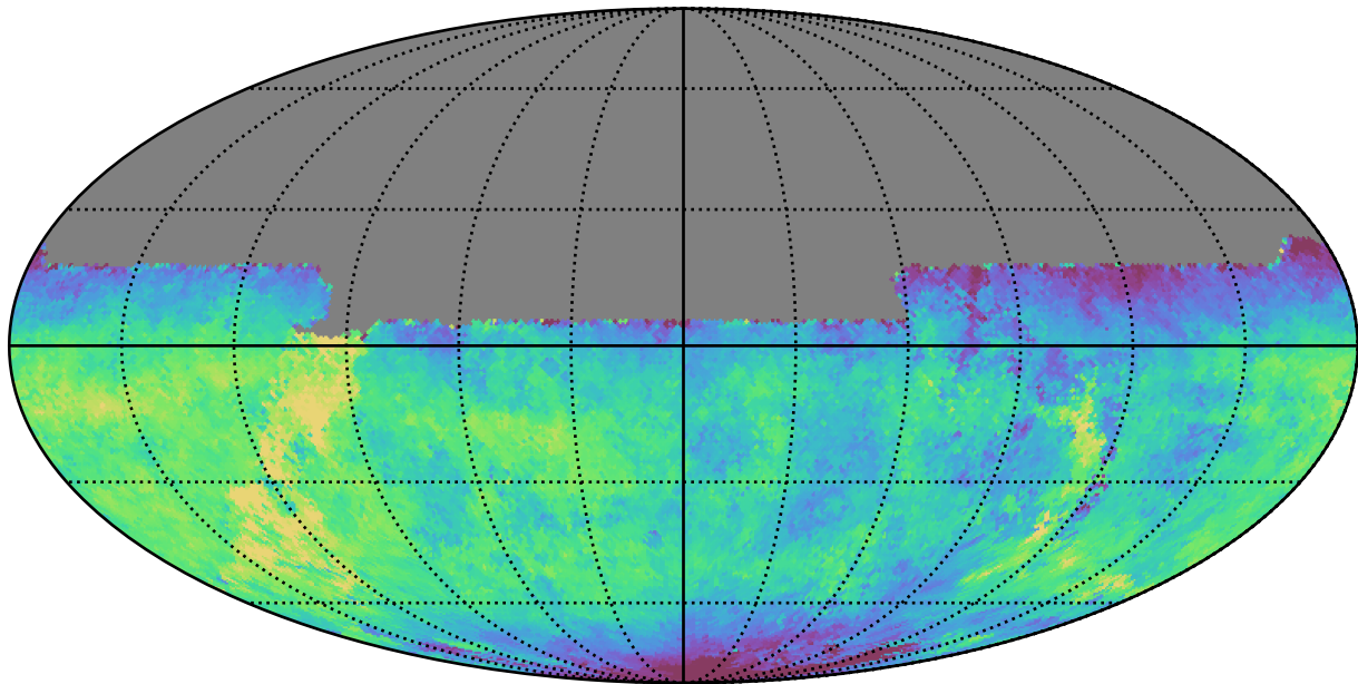
too_100_1v3.4_10yrs All sky u band: Median saturation_mag
