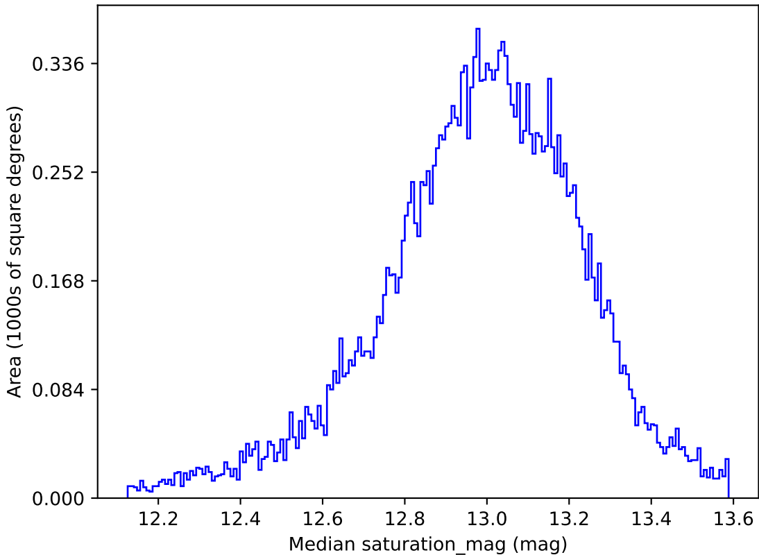
too_100_1v3.4_10yrs All sky u band: Median saturation_mag
