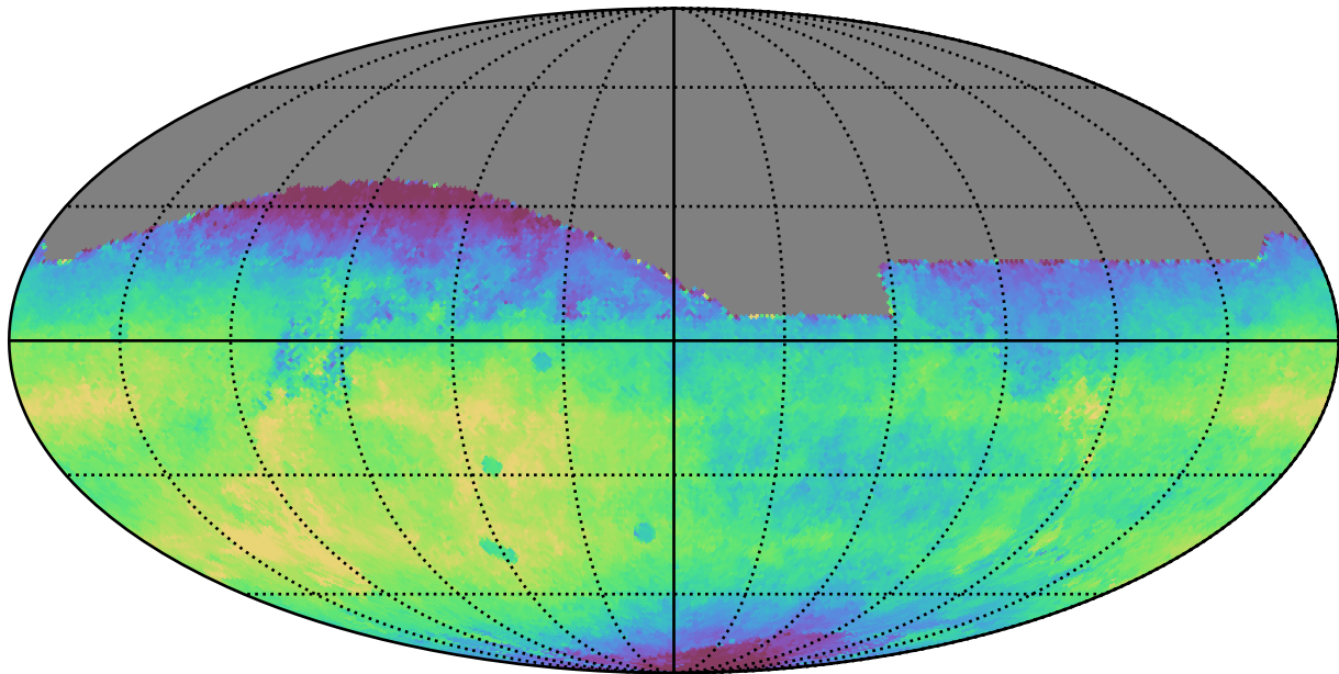
too_100_1v3.4_10yrs All sky r band: Median saturation_mag
