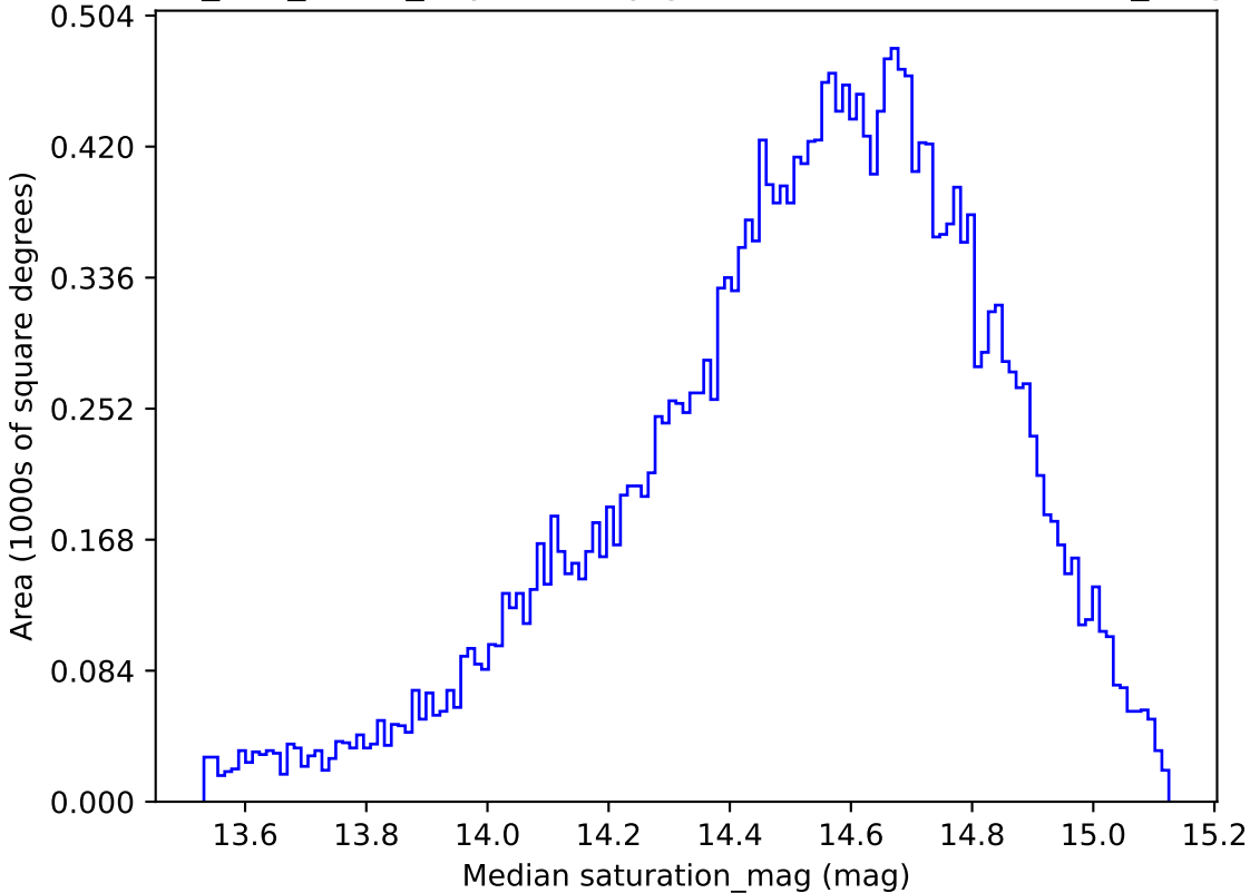
too_100_1v3.4_10yrs All sky g band: Median saturation_mag
